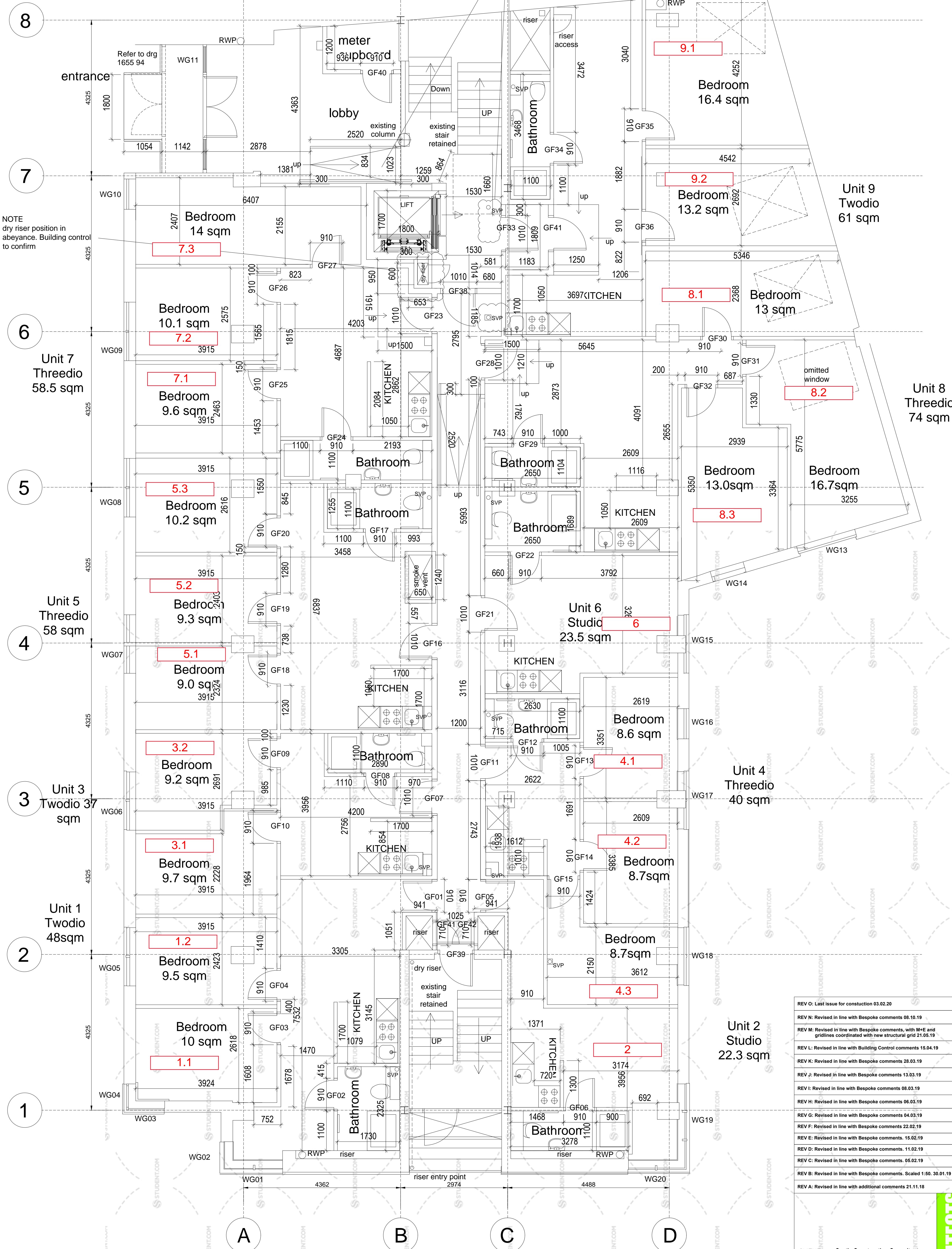
Proposed ground floor
